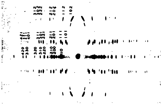
FIG. 5.—Rotation photograph of a tetragonal crystal of urea about the [001] axis. Unfiltered copper radiation. Cylindrical film.
